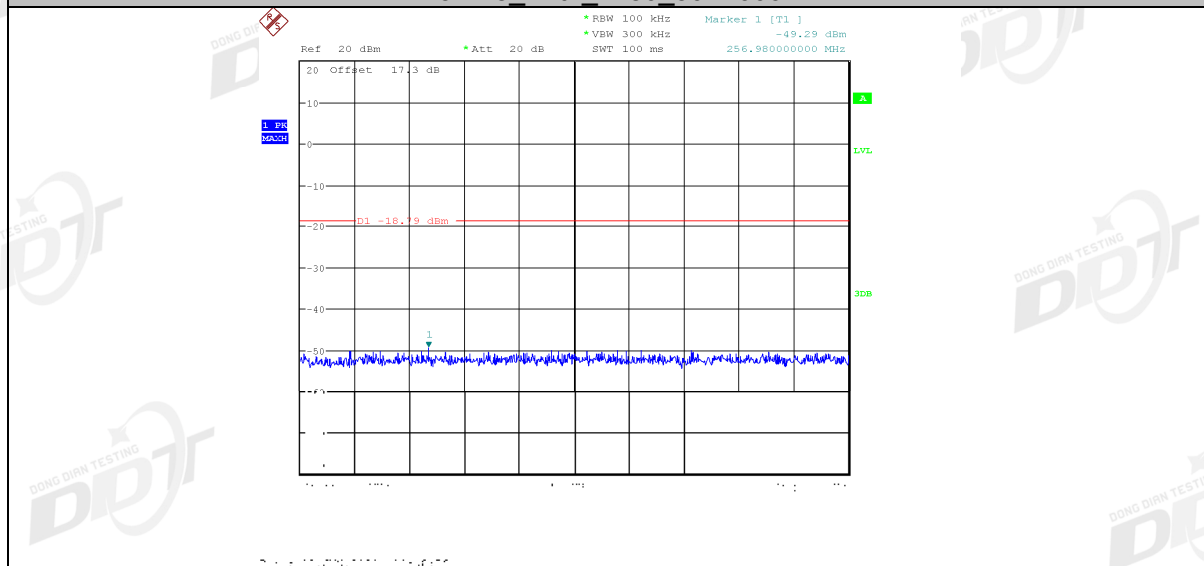
3DH5_Ant1_2480_1000~26500
