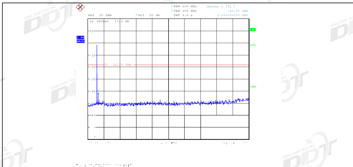
3DH5_Ant1_2480_0~Reference
