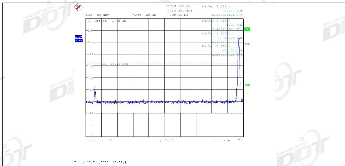
2DH5_Ant1_High_2480
